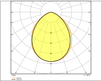
FL COMP V 10W 830 SYM 100 BK
