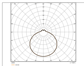
SF CIRC 350 V 18W 3CCT IP44
