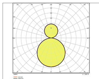
PANEL D/I 1200 36 W 3000 K UGR19
